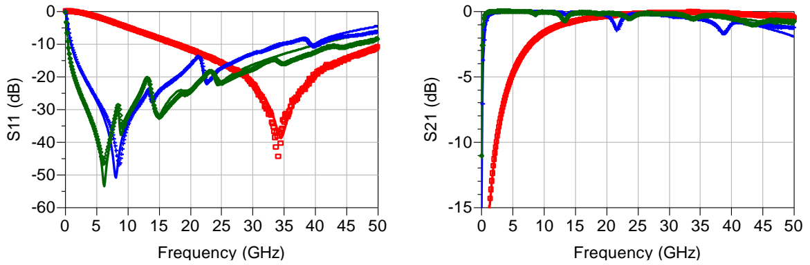
6.6 mil Rogers 4350B (H/Er = 1.5 mil):
