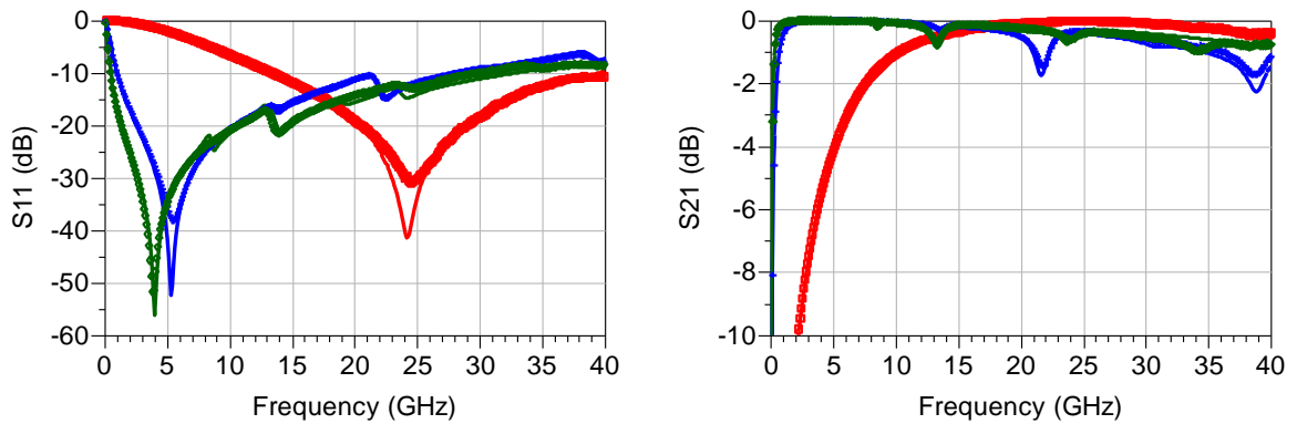
10 mil Rogers 4350B (H/Er = 2.6 mil):
