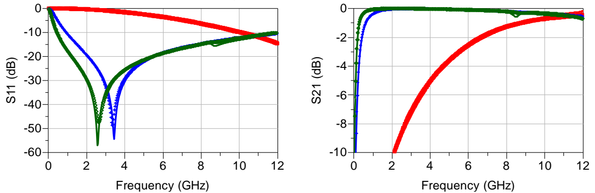
30 mil Rogers 4350B (H/Er = 8.6 mil):
